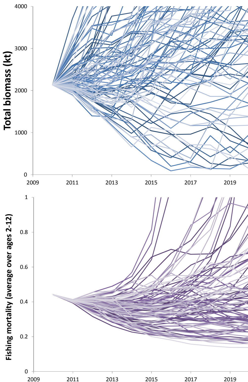
Figure 16. Stochastic projections of biomass (kt; top panel) and fishing mortality (average 2-12; bottom panel) for the base case model (Model 4) under the assumption that future recruitment has the same mean and variance as the 10-year period 2000-2009 and assuming constant catch of 711 kt (equal to the 2010 catch).
