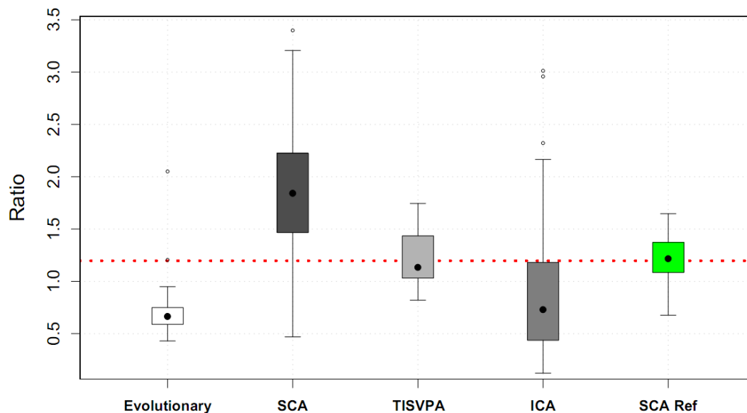
Figure 7. Recent trend in spawning stock size computed as the ratio of 2007 over 2000 relative to the true underlying population value (horizontal line). The first and third quantile of each dataset are represented by the shaded boxes, while minimum and maximum observations, not being outliers, are represented by the dotted vertical lines. Outlying results (more than 1.5 times the interquartile distance away from the 1st or 3rd quantile) are represented by open circles.
