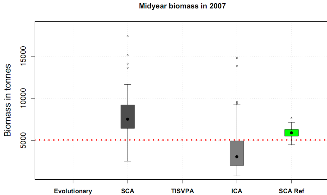
Figure 6. Total mid-year biomass in 2007 compared to the true underlying population value (horizontal line). The first and third quantile of each dataset are represented by the shaded boxes, while minimum and maximum observations, not being outliers, are represented by the dotted vertical lines. Outlying results (more than 1.5 times the interquartile distance away from the 1st or 3rd quantile) are represented by open circles.
