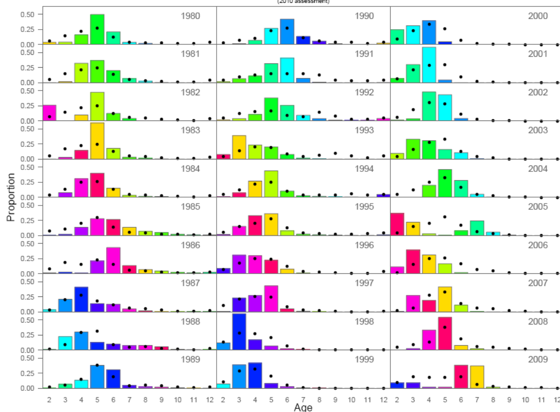
Figure 4. Base case (model 4) fit to the age compositions for the far north fishery (Fleet 3). Bars represent the observed data and dots represent the model fit and color codes correspond to cohorts.
