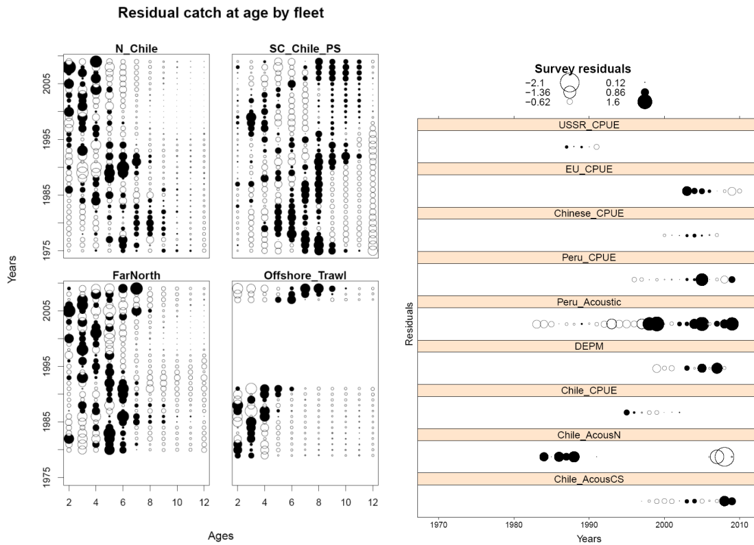
Figure 4. Logged residuals of observed and predicted catch-at-age proportions for the different fleets (left) and residuals for each of the indices (right) from JJM model 4.
