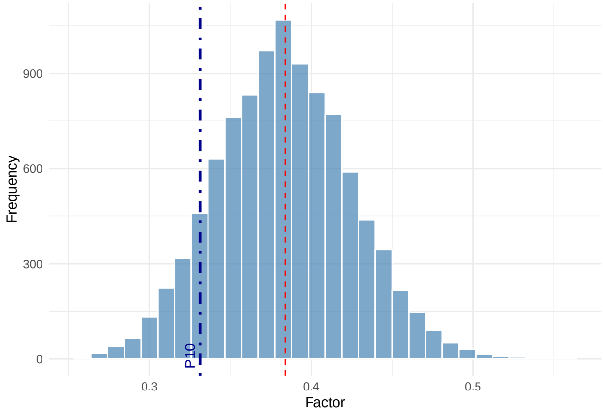
Figure 1: Unweighted bootstrap distribution of the survey technological improvement factor.
